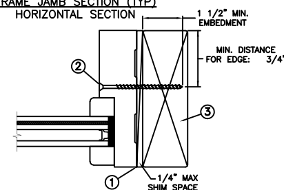
FRAME JAMB SECTION (TYP) HORIZONTAL SECTION
