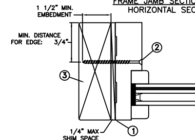
FRAME JAMB SECTION (TYP) HORIZONTAL SECTION
